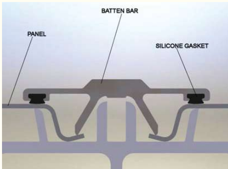
Fig. 1 – AluminumDomes.com Detail
