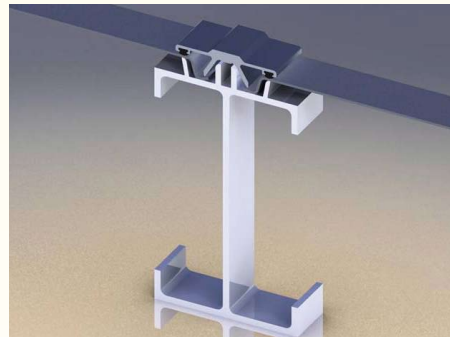
Fig. 2 – AluminumDomes.com Detail
